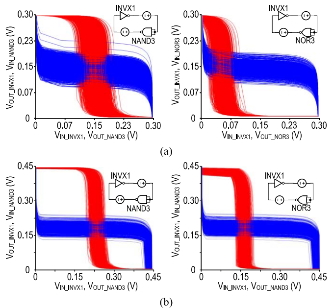
Fig. 5. Noise margin verification versus NAND3 and NOR3 from layout extractions with (a) 0.30 V and (b) 0.45 V operations.
