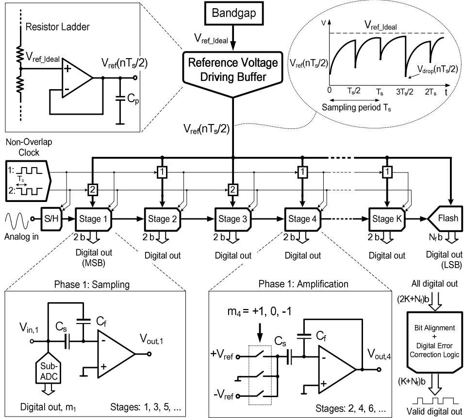
Fig. 1 A generic switched-capacitor 1.5-bit/stage pipelined ADC. The number of pipelined stage, K , is assumed to be even
