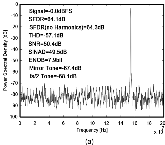
Fig. 4 Power spectral density (non-ideal model simulation). (a) With infinite V_{ref} precision. (b) With 6-bit V_{ref} precision
