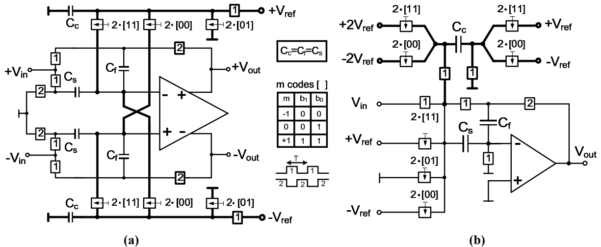
Fig. 7 (a) Weighted-summer V_{ref} compensation. (b) Correlated double-sampled V_{ref} compensation.
