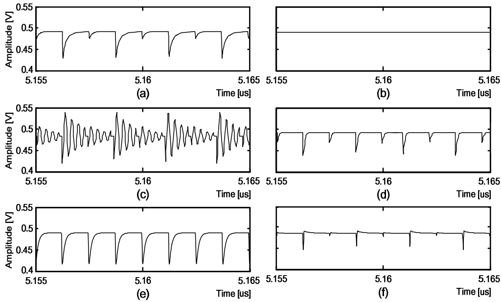
Fig. 6 Simulated reference voltages. (a) No stabilization. (b) With 1000-pF stabilization capacitor on-chip. (c) With 1000-pF stabilization capacitor off-chip. (d) Case (c) with another 100- \Omega resistor added in series. (e) Proposed on-chip V_{ref} compensation method 1. (f) Proposed on-chip V_{ref} compensation method 2.
