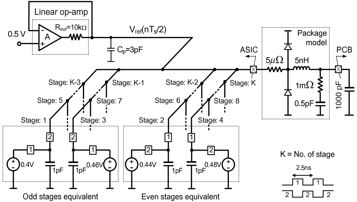
Fig. 5 A two-phase equivalent-circuit model of V_{ref} generation in pipelined ADC.
