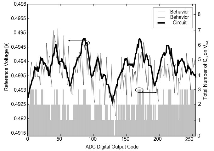
Fig. 3 Behavior and circuit simulation results of V_{ref} .
