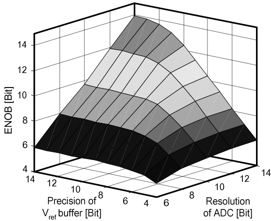
Fig. 2 Reference voltage buffer precisions versus ENOBs for different ADC resolutions.
