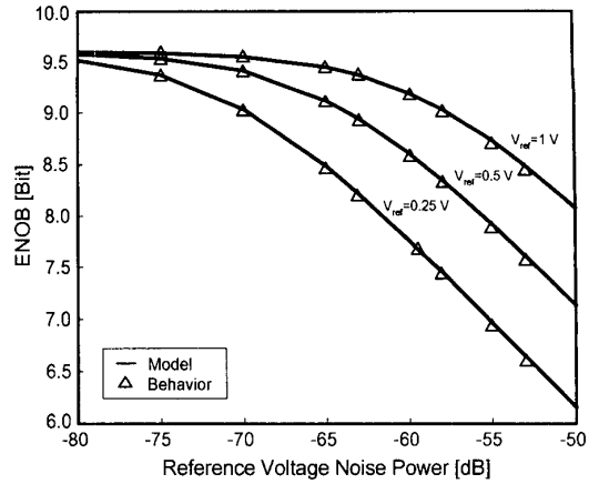
Fig. 10. ENOB as a function of noise power and its input-referred noise. (-1-dBFS input and 10-bit resolution are assumed).
