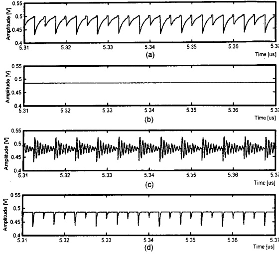
Fig. 3. V_{ref} fluctuation in four cases. (a) With no stabilization capacitor. (b) With 1000-pF stabilization capacitor on-chip. (c) Off-chip implementation of case (b). (c) With added 100- \Omega resistor.
