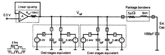
Fig. 2. Equivalent model of V_{REF} generator with and without off-chip stabilization capacitor.
