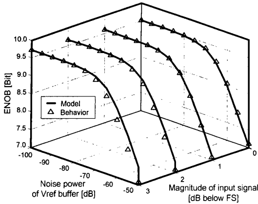
Fig. 9. ENOB as a function of noise power and input magnitude. (10-bit resolution and 0.5-V reference voltage are assumed.)
