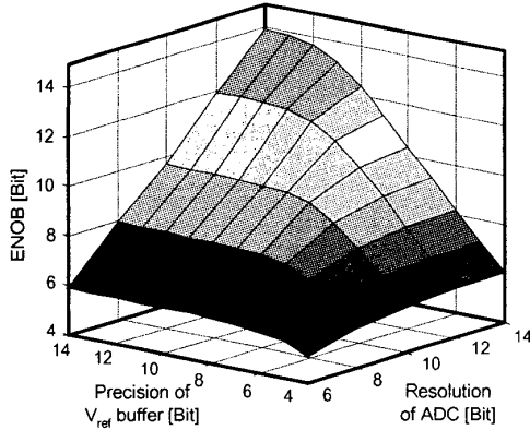
Fig. 4. Influence of reference voltage buffer precision on ENOB for different ADC resolution.
