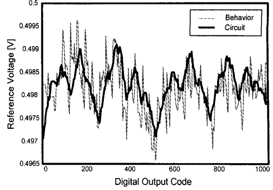
Fig. 5. Reference voltages obtained through behavioral model and schematic simulations.
