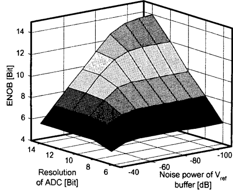
Fig. 8. Influence of reference voltage noise on ENOB for different ADC resolution.
