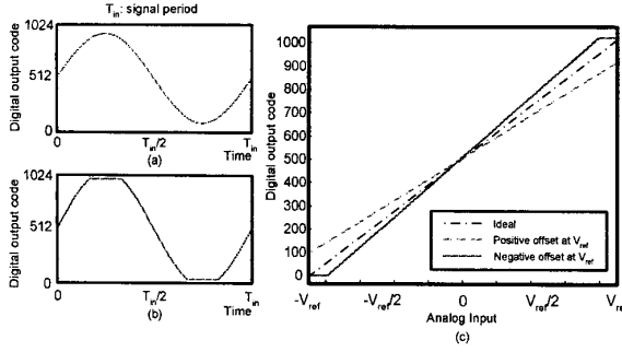
Fig. 6. Time domain of (a) Positive offset. (b) Negative offset. (c) Their corresponding A/D conversion curves.
