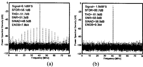
Fig. 7. (a) Influence of offset voltages to the SFDR and ENOB performance of the entire ADC. (a) Negative. (b) Positive.
