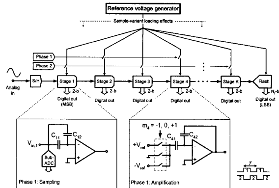
Fig. 1. A generic 1.5-bit/stage pipelined ADC.
