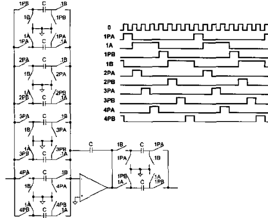
Fig.3 One path of the 4-path comb-filter plus integrator
