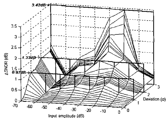
Fig.7 Monte Carlo simulation shows \Delta S\text{NDR} within different deviation \sigma , 2\sigma and 3\sigma , where \sigma=0.2\%
