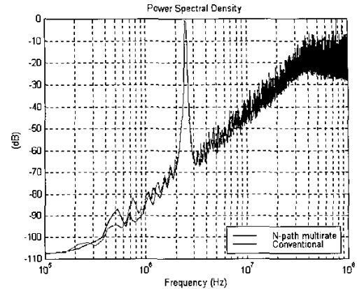
Fig.5 Output spectrum for a -10dB 2.5MHz input sine-wave at 216MHz sampling frequency
