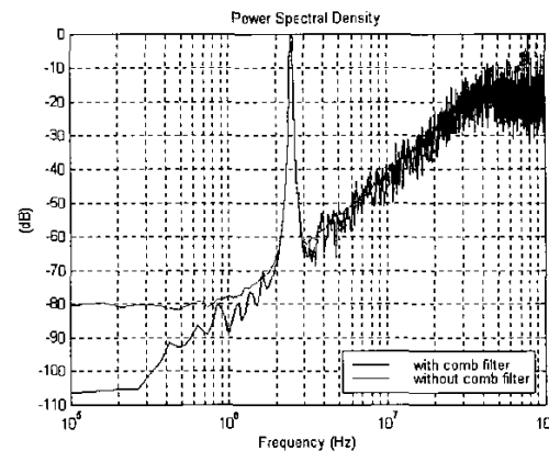
Fig.6 Output spectrums with 0.4% coefficient mismatch by using comb filter versus no comb filter
