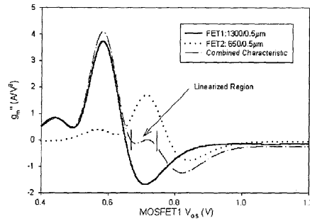
Fig. 3 g_m'' Cancellation by 2 MOSFETs
