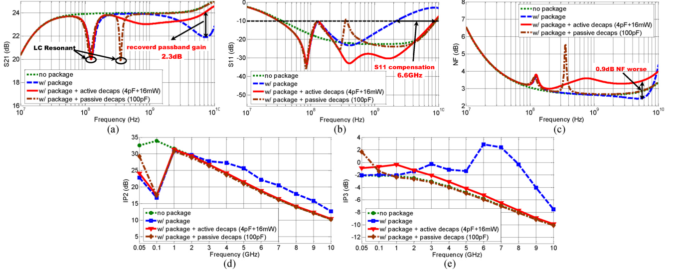
Fig. 6. Simulation results for (a) S21, (b) S11, (c) NF, (d) IP2, (e) IP3.
