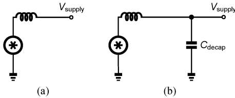
Fig. 3. (a) Noisy power supply in the presence of package inductance, (b) noise suppression by applying decaps.
