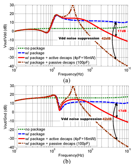
Fig. 7. Noise filtering performances for (a) voltage supply, (b) ground.
