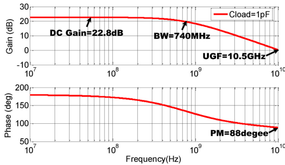
Fig. 5. Simulated bode plot of the active decap opamp.
