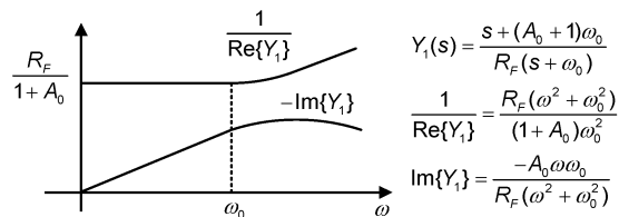
Fig. 8. Behavior of Y_1 components with frequency.
