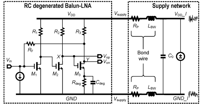
Fig. 1. RC-degenerated balun-LNA and practical supply network model.
