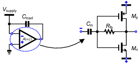
Fig. 4. Schematic of proposed active decap circuit.
