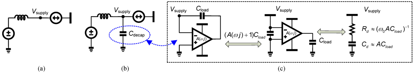
Fig. 2. (a) Circuit performance degradation due to package parasitics, (b) package effects cancellation by decaps, (c) active decaps principle.
